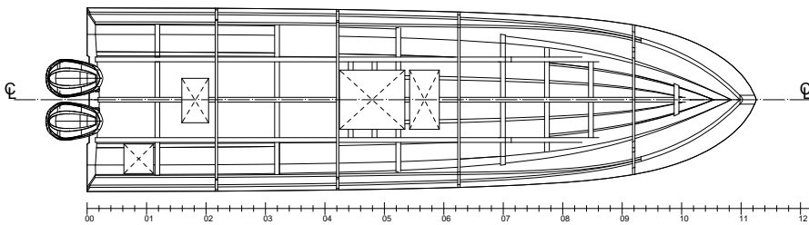
LOWER DECK
